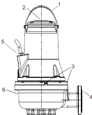
Fig. 1 FK pump
