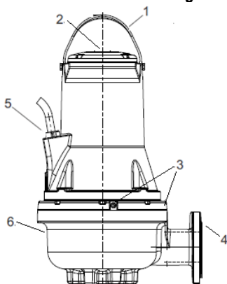
Abb. 1 FK- Pumpe
